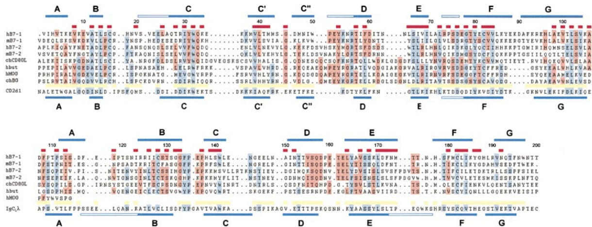
Figure 2. Alignment of B7 Subset and Human CD2 d1 and IgC 1 λ Sequences Based on the sB7-1, sCD2, and IgG1 λ Light Chain Crystal Structures
